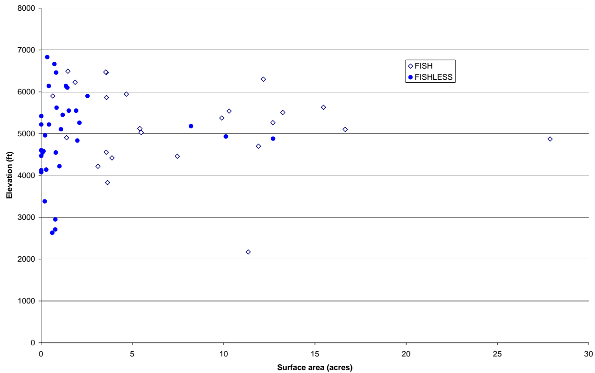
FIGURE 18. Distribution of fishless and fish inhabited waters with respect to surface area and elevation where long-toed salamander ( A. macrodactylum ) have been observed.
